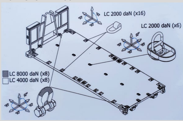
LASHING POINT LAYOUT
